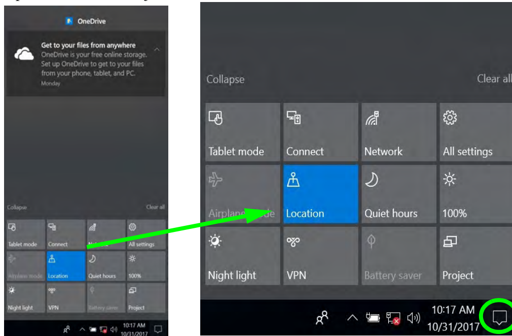
Figure 1 - 21 - Action Center
