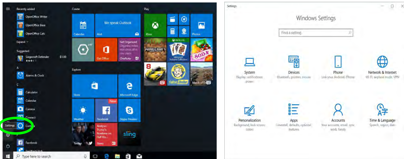
Figure 1 - 19 - Settings
