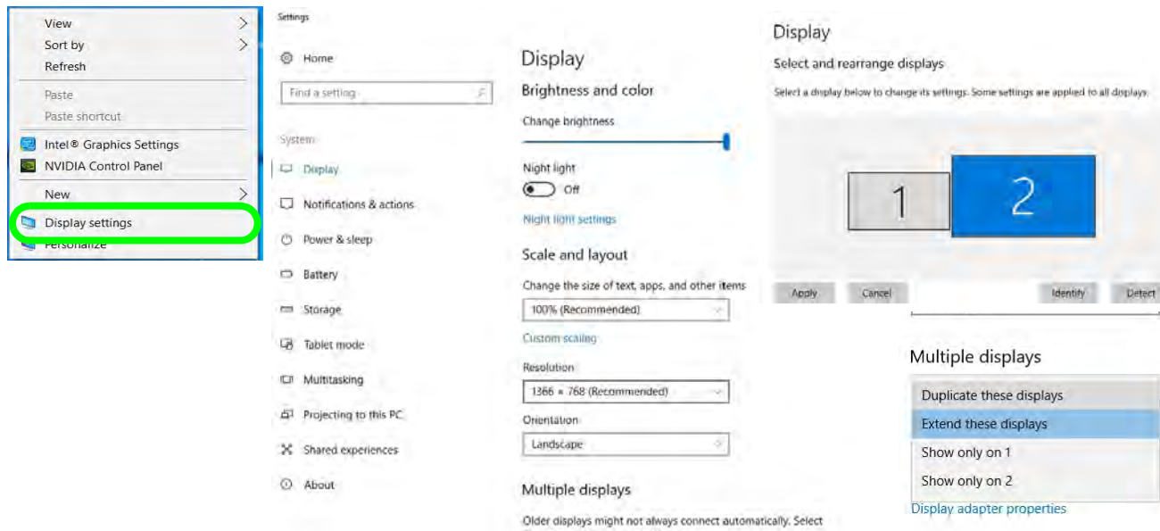
Figure 1 - 23 - Display Settings
