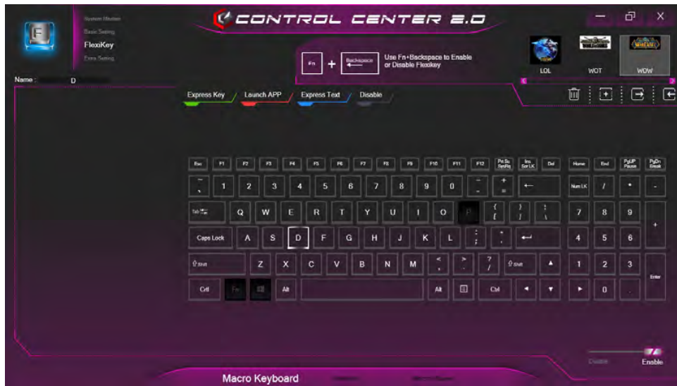
Figure 1 - 6 - Flexikey® Application
